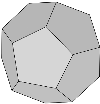
dodecahedron
