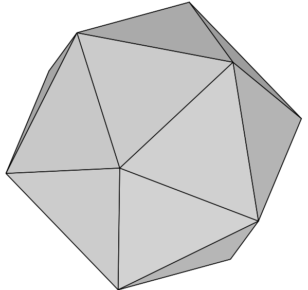
icosahedron
