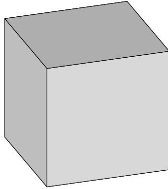
hexahedron
