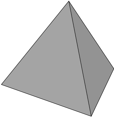
tetrahedron
