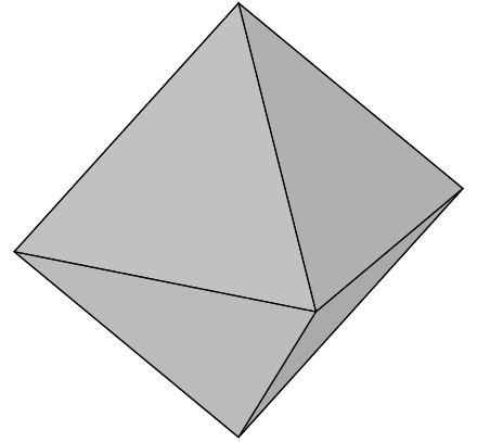
octahedron
