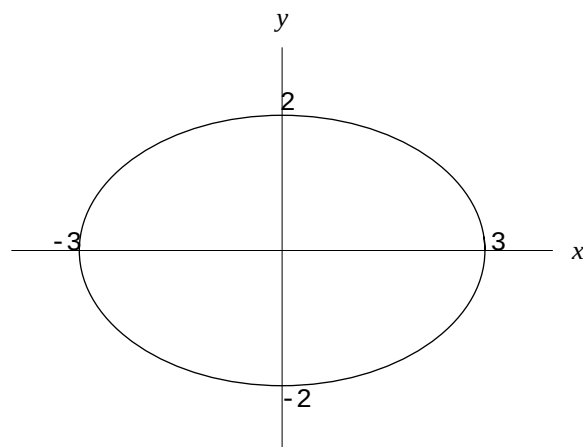
図 3: \frac{x^2}{9} + \frac{y^2}{4} = 1
