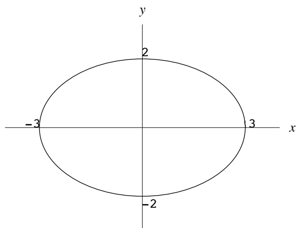
図 3: \frac{x^2}{9} + \frac{y^2}{4} = 1
